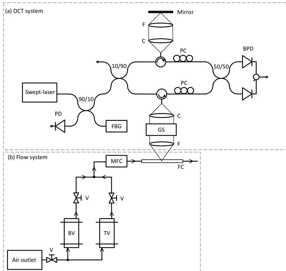
Fig. 1. Schematic of the experimental swept-source OCT set-up (a) and flow system (b). PD: photodetector, FBG: fiber Bragg grating, PC: polarization controllers, C: collimating lens, F: focusing lens, GS: galvanometric scanner, FC: flow channel, TV: tracer vessel, BV: bacteria vessel, V: valve, and MFC: mass flow controller. Adapted from Ref. [22].
