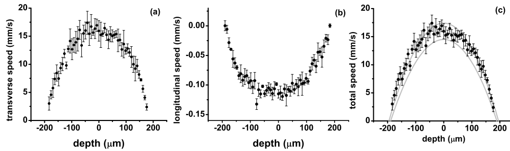
Fig. 4. Measured flow velocities at the center of the flow channel: (a) transverse flow velocity, (b) longitudinal flow velocity, and (c) total flow velocity. The parabolae show the confidence interval of the reference flow velocity calculated based on the set-point of the mass-flow controller and the measured channel depth and width.
